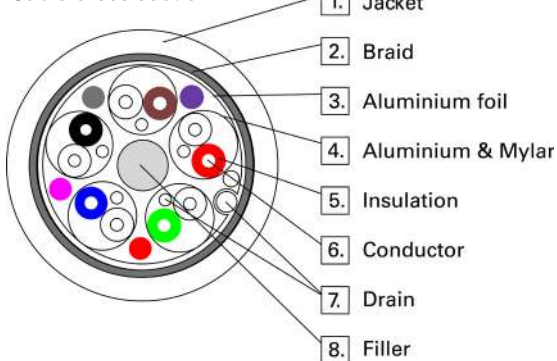
Cable cross section:
